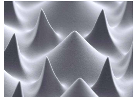
Diffuser: Resist AZ 4562, structure size < 5 μm
