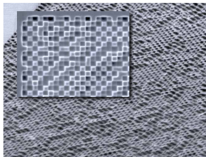
DOE: Resist AZ 4633, resist thickness 4 μm, structure size 2 μm
