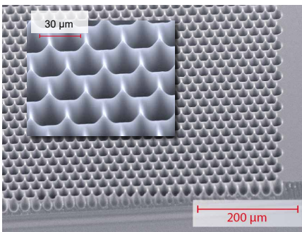
Microlens array: Width of lenses 20 μm, depth 30 μm
